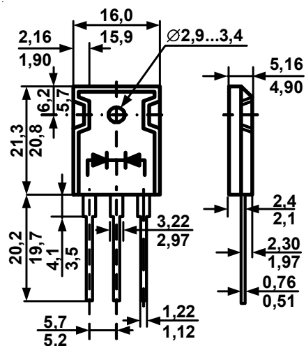
TO-3P
