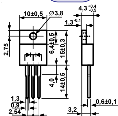
TO-220
