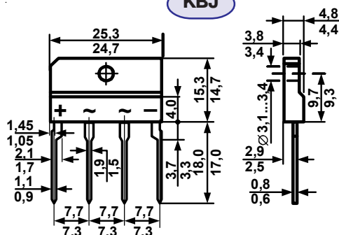
KBJ
