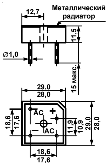
BR-25W
